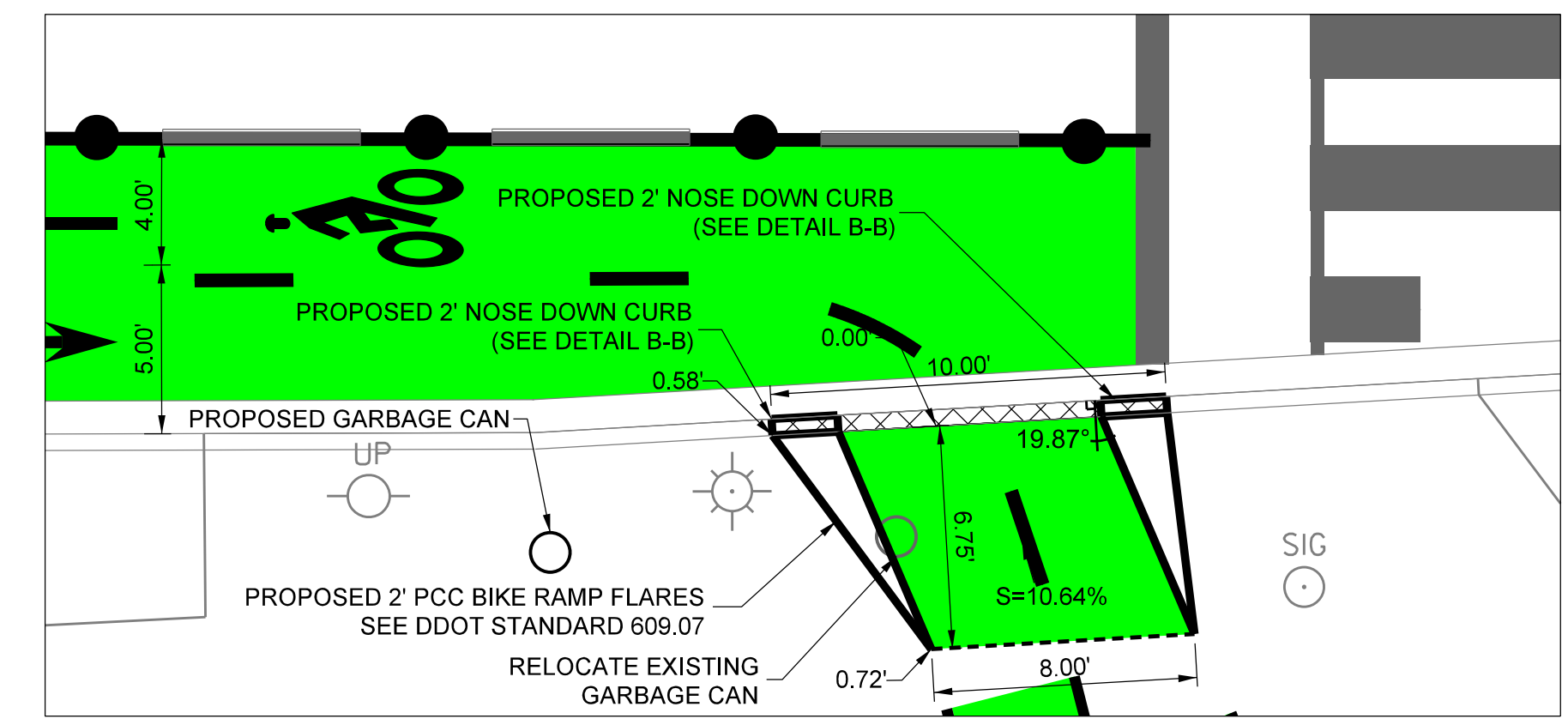
2 CYCLE TRACK RAMP ELEVATION DETAILS SCALE: 1"=10'
