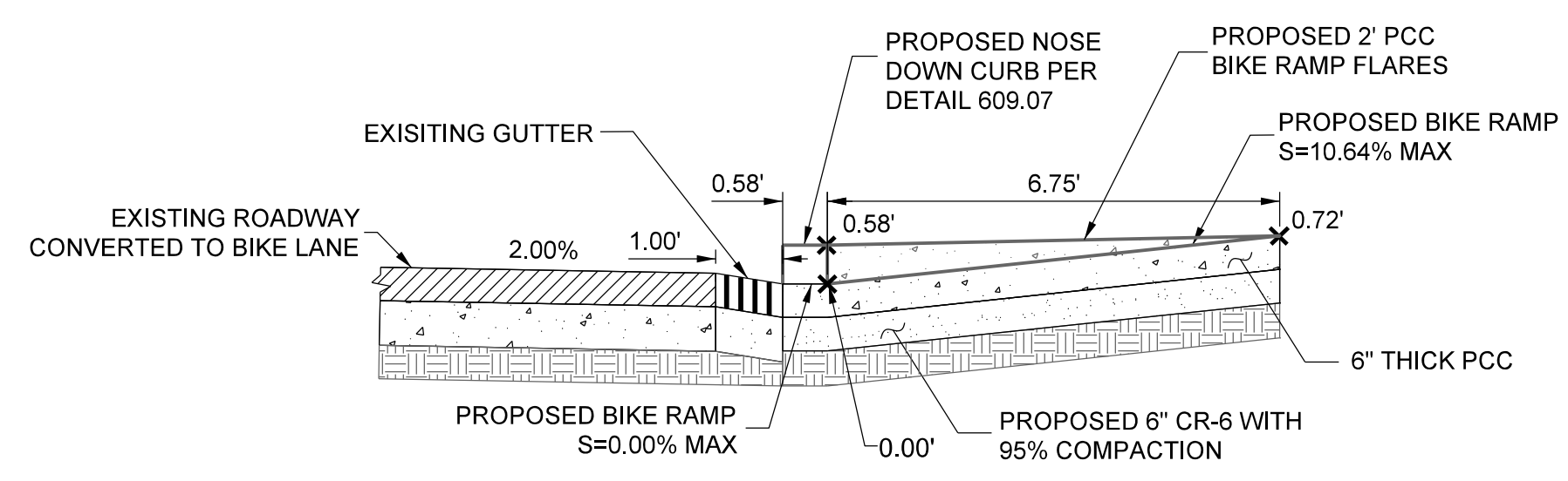
A-A CYCLE TRACK RAMP SECTION SCALE: 1" = 5'
