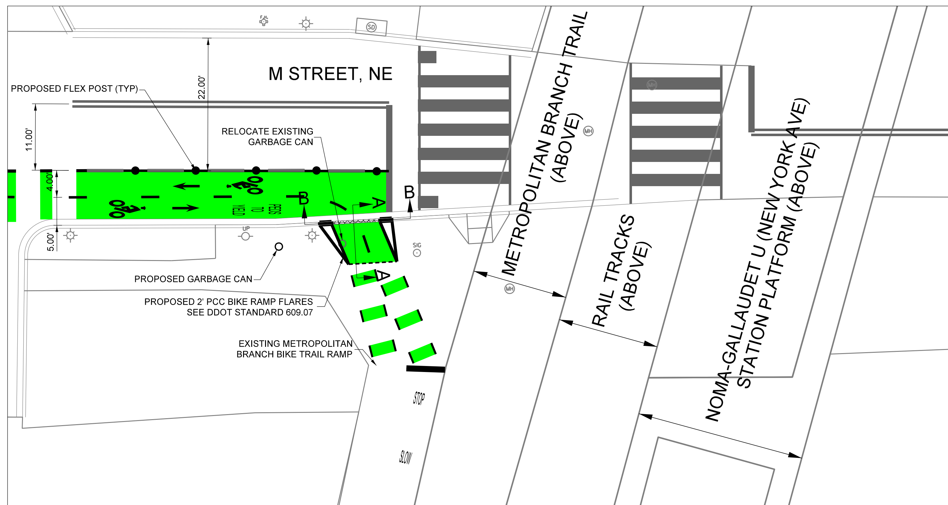
1 CYCLE TRACK RAMP PLAN VIEW SCALE: 1"=20'
