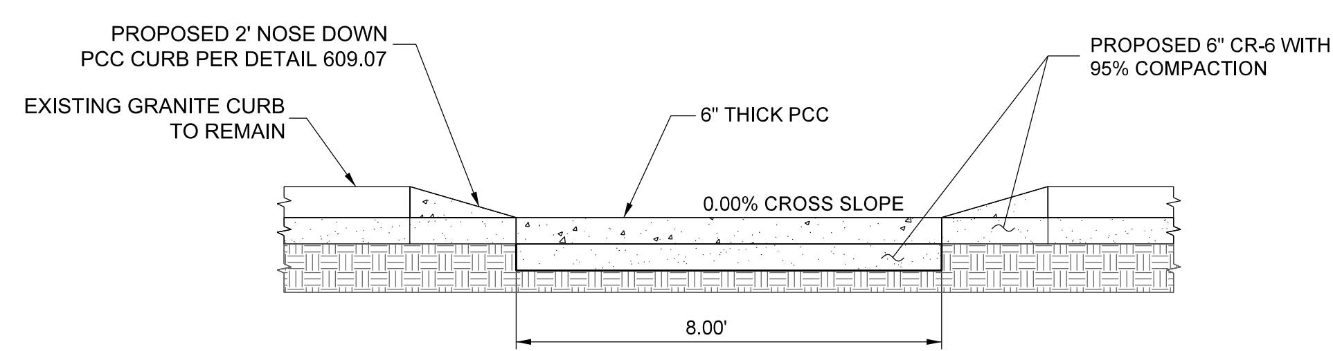
B-B CYCLE TRACK RAMP CROSS SECTION SCALE: 1" = 5'
